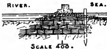
FIG. 4.—Mississippi South Pass Outlet Jetty.
