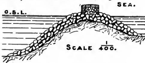
FIG. 3.—Lido Outlet Jetty, Venice.
