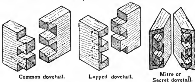
FIG. 3.—Dovetails.
