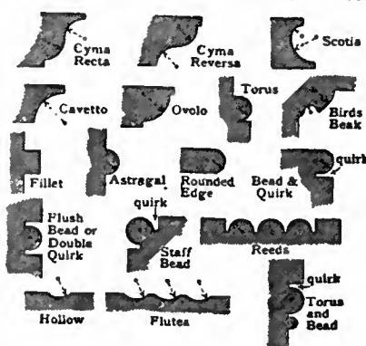
FIG. 5.—Mouldings.
