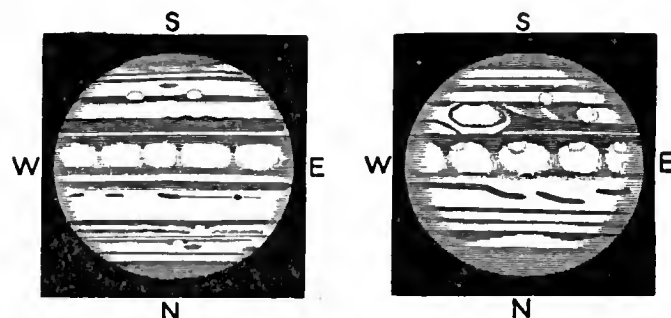
FIG. 2.—Jupiter, 1903, July 10, 2:50 a.m.
