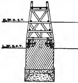
FIG. 2.—Dunkirk East Jetty.
