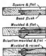
FIG. 11.—Forms of Panelling.
