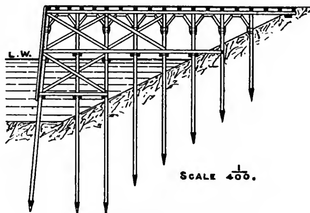
FIG. 1.—Timber Jetty across Dock Slope.
