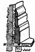
FIG. 6.—Built-up Skirting tongued to floor.
