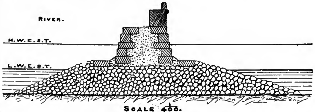
FIG. 6.—River Nervion Outlet, Western Jetty.
