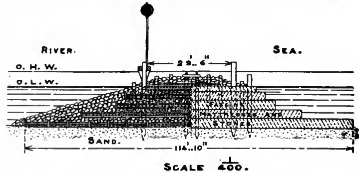
FIG. 5.—River Maas Outlet, North Jetty.
